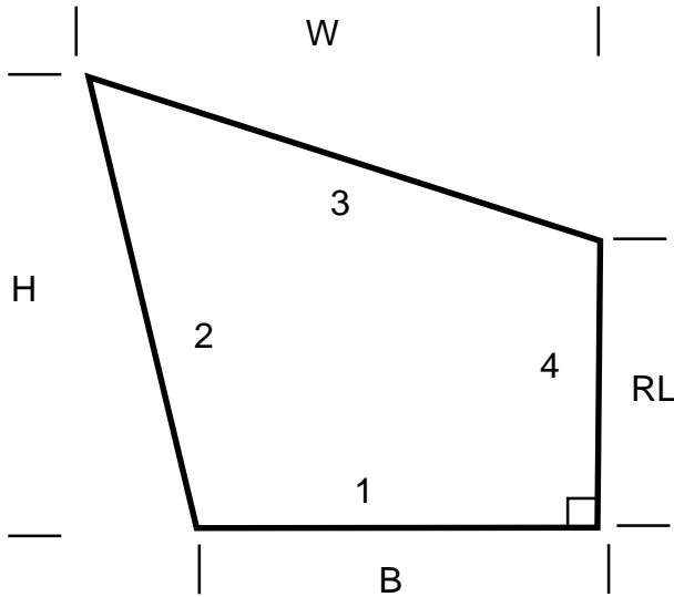
shape #11 IRREGULAR GABLE RH
