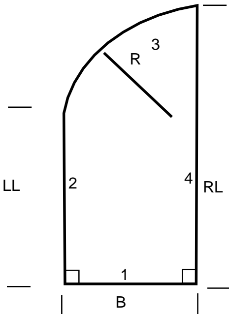
shape #67 ARCH GABLE LH
